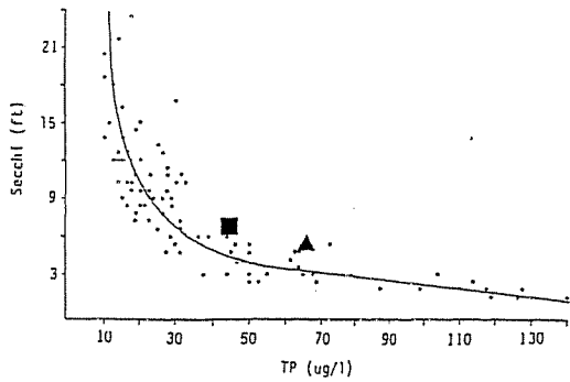
SCATTERPLOTS OF CHLOROPHYLL-a, SECCHI TRANSPARENCY, AND TOTAL PHOSPHORUS. Based on summer mean concentrations for ecoregion lakes.
