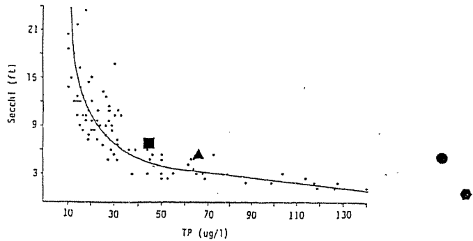
SCATTERPLOTS OF CHLOROPHYLL-a, SECCHI TRANSPARENCY, AND TOTAL PHOSPHORUS. Based on summer mean concentrations for ecoregion lakes.
