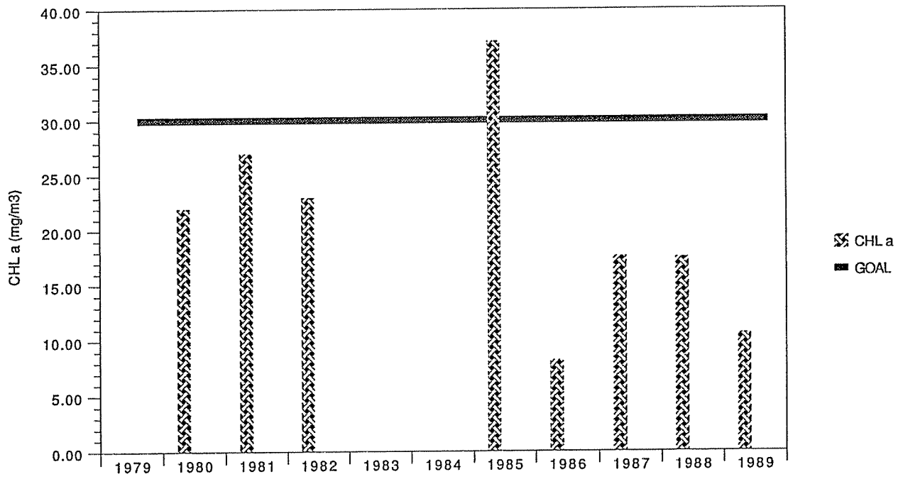
Chlorophyll a
