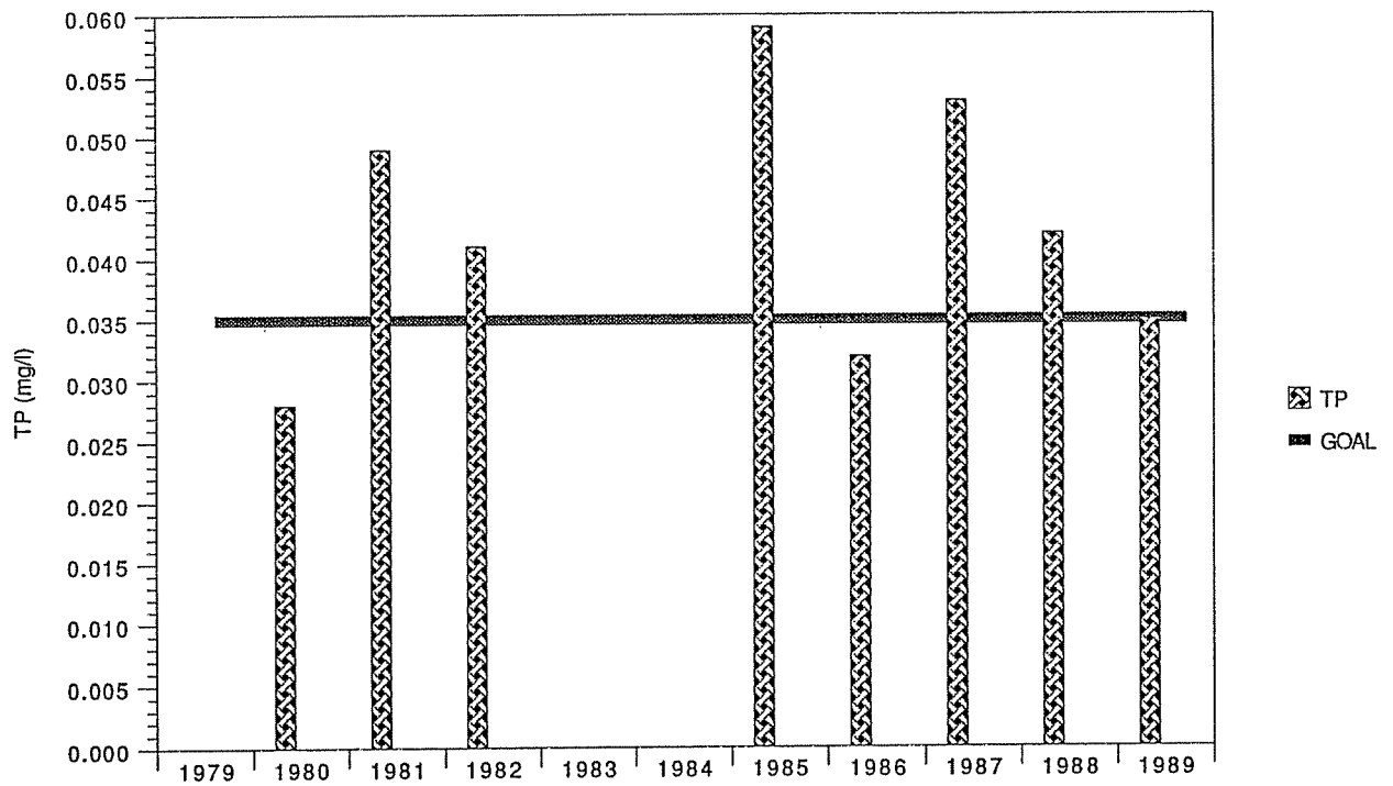
Total Phosphorus
